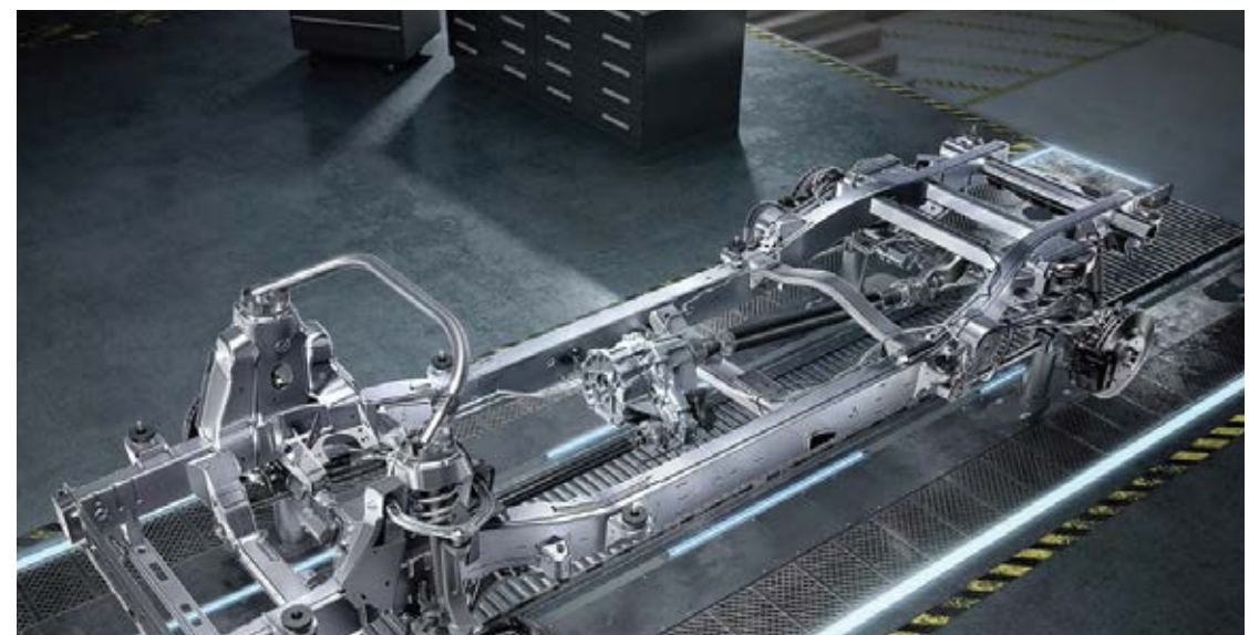
AMG ACTIVE RIDE CONTROL Suspension
